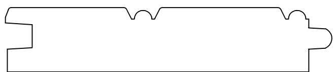
\frac{9}{16} " x 3\frac{1}{4} " Beaded Ceiling Moulding
